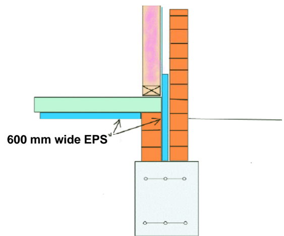
Slab Edge Insulation Detail for Strip Footing Slab On-ground Construction
